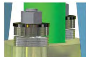
Live-loading Detail
