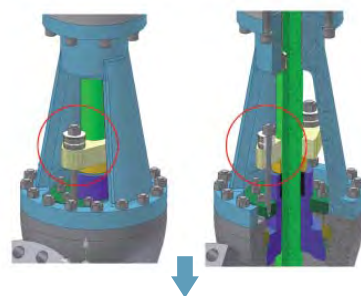
Live-loading
