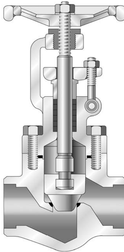
Bolted Bonnet
